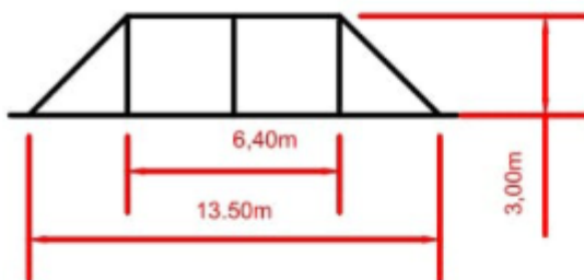
Vista frontal
